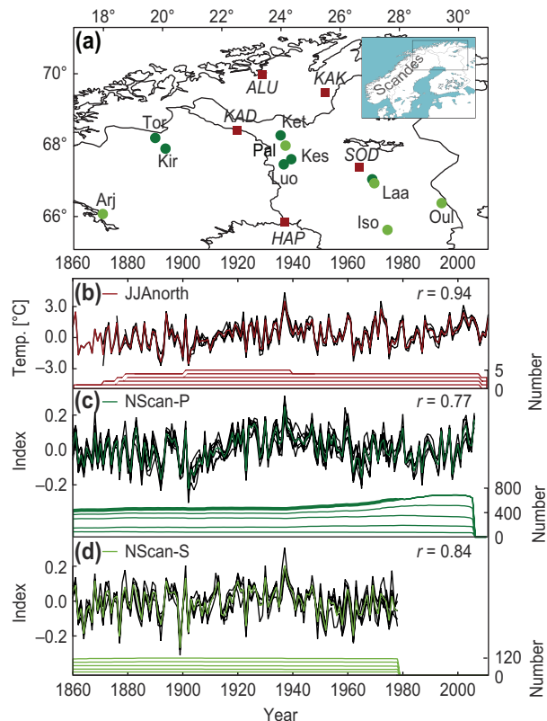
Figure 1. Fennoscandian temperature and MXD records. (a) Location of five meteorological stations (red), six Pinus sylvestris (dark green, Tor including Tor-old) and five Picea abies (light green) MXD sites in Northern Fennoscandia. (b) JJA temperatures recorded at the five stations (black) and their arithmetic mean (red). Bottom panel shows the station replication. (c) and (d) Pinus sylvestris and Picea abies site chronologies (black) and their arithmetic means (pine in light green, spruce in dark green). Bottom panels indicate the replication (number of MXD measurement series) of the site chronologies. Correlation coefficients in (c)–(d) were calculated over the common 1879–1978 period.
