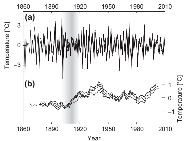
Figure 4. High- and low-pass filtered northern Fennoscandian summer temperature records. (a) First-difference timeseries of JJA temperatures recorded at five stations in northern Fennoscandia (see Fig. 1a for locations). (b) Same as in (a), but after low-pass filtering the original timeseries using 15-year running means. Low-pass filtered anomalies refer to the 1890–1930 period. EDP is highlighted with grey shading.
